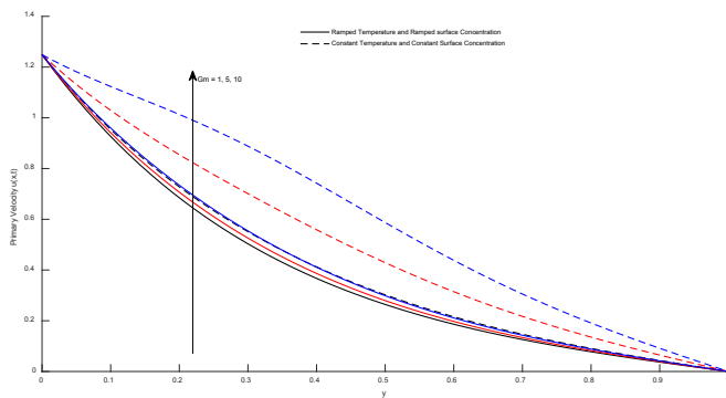
Figure 7. Graph of Primary velocity Vs the heat transfer Grashof number Gr
