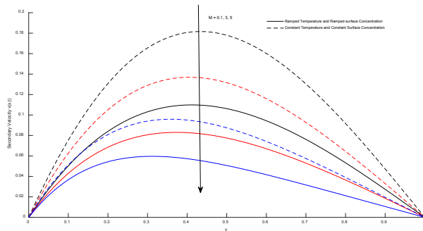
Figure 11. Graph of Secondary velocity v(x,t) Vs the magnetic fluid parameter M
