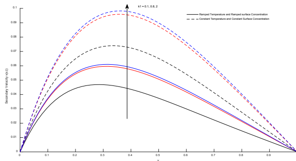
Figure 12. Graph of Secondary velocity v(x,t) Vs the permeability parameter k_1
