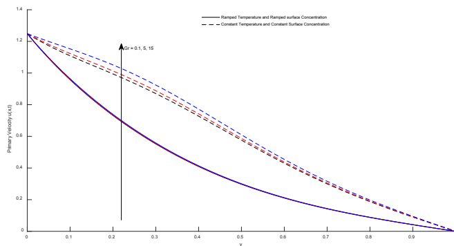
Figure 8. Graph of Primary velocity Vs the mass transfer Grashof number Gm
