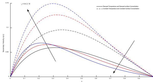
Figure 10. Graph of Secondary velocity v(x,t) Vs the Casson fluid parameter \gamma
