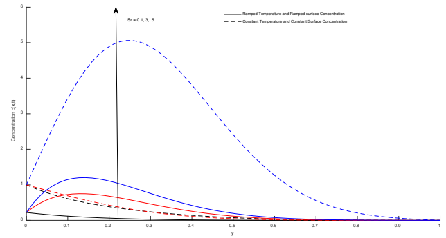
Figure 18. Graph of the concentration profile C(x,t) Vs the Soret parameter Sr
