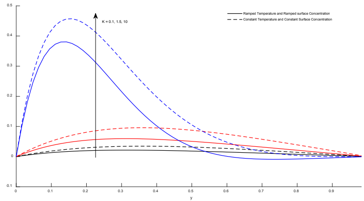
Figure 13. Graph of Secondary velocity v(x,t) Vs the rotation parameter k
