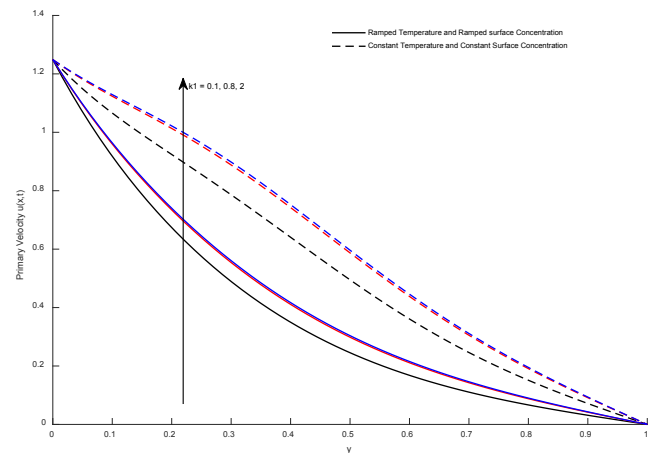
Figure 5. Graph of Primary velocity Vs the permeability parameter k_1
