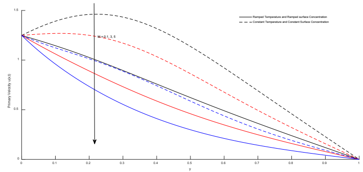
Figure 4. Graph of Primary velocity Vs the Magnetic fluid parameter M
