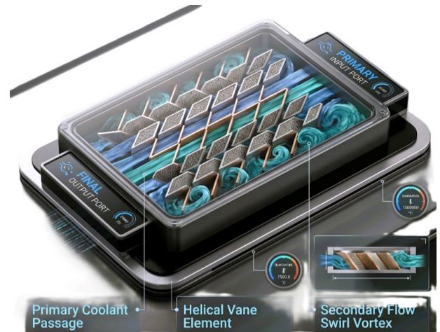
Figure 16. Illustration of plan view of heat sink with oblique fins
