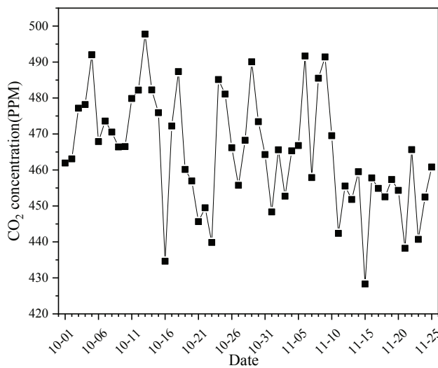
Figure 7. Daily average carbon dioxide concentration monitored by carbon flux tower.
