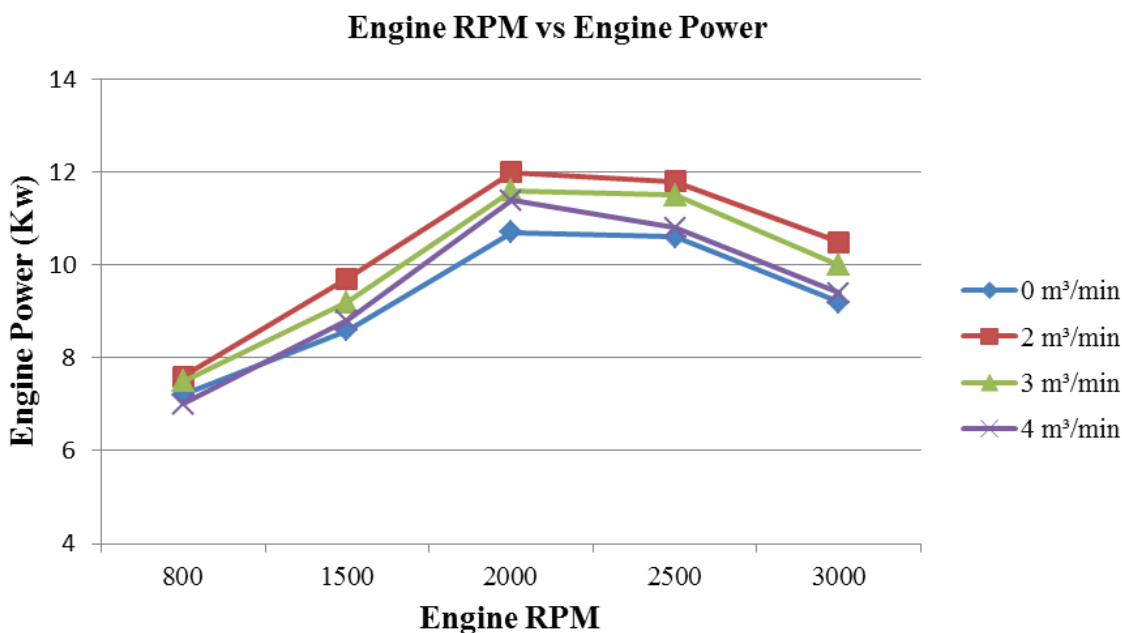
Figure 7. Variation of engine power with engine rpm for different flow rate of fresh air in exhaust system.
