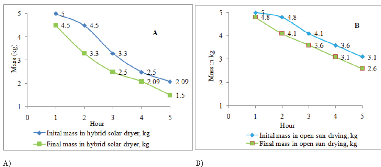
Figure 13. Initial and final mass of mangoes for five hours during the drying process. A. hybrid solar drying B. Open sun drying.
