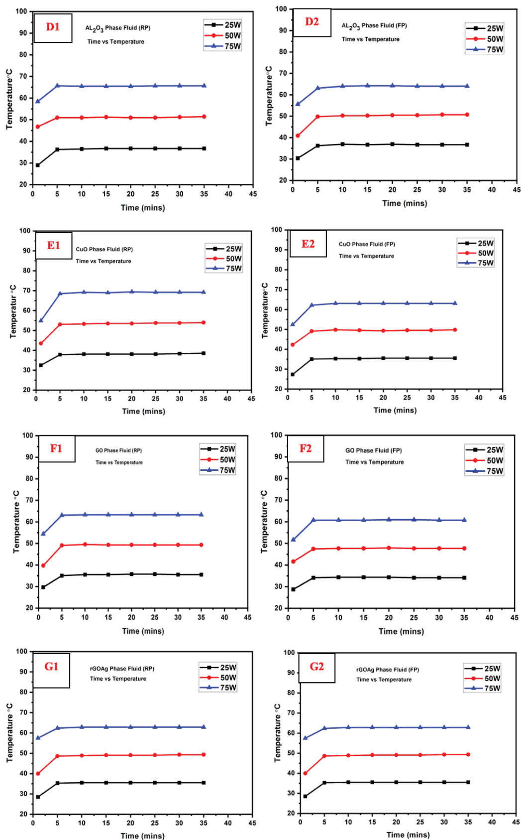
Figure 7. (A1-A2), (B1-B2), (C1-C2), (D1-D2), (E1-E2), (F1-F2) and (G1-G2) represents Graph of time Vs heater temperature for without any interfacial material, paraffin wax, SiO_2 , Al_2O_3 , CuO, GO, rGO at difference power inputs of 25W, 50W and 75W and at full pressure (FP) and reduced (RP).
