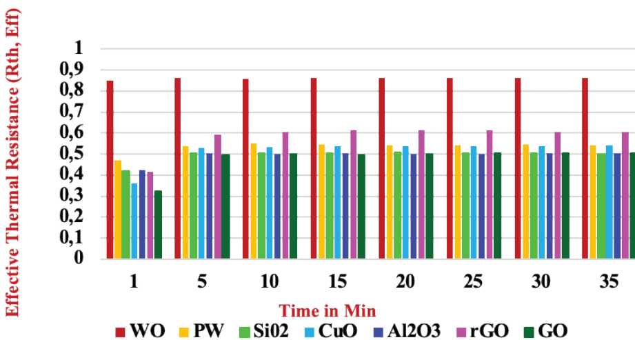
Figure 9. Comparison of different TIM at 50 W input power at reduced pressure.
