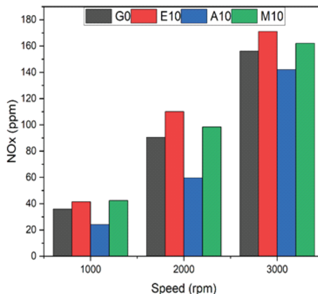
Figure 10. NO x emissions vs. engine speed.
