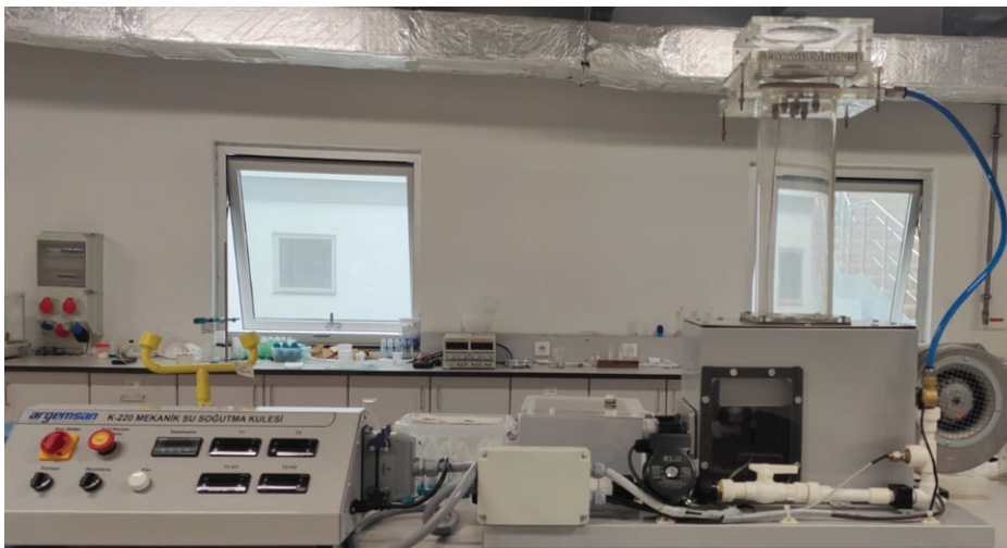
Figure 2. The laboratory scale mechanical draft cooling tower.
