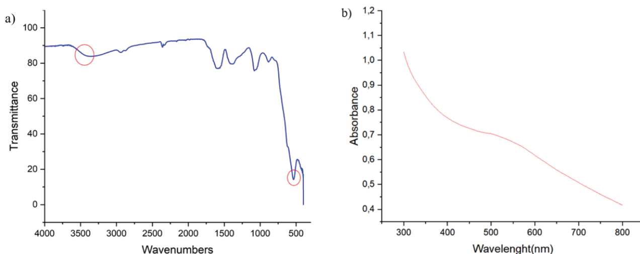
Figure 3. FTIR spectrum of synthesized nanoparticles (a), and their corresponding UV- Vis spectrum (b).
