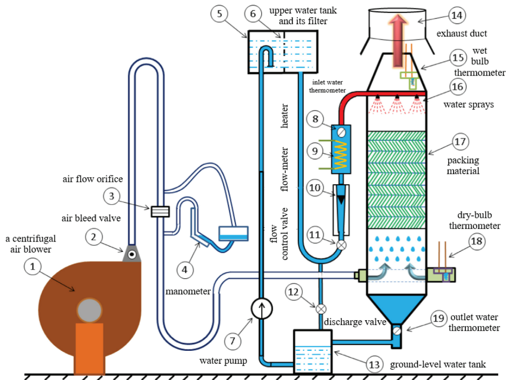
Figure 1. A Schematic diagram of the experimental setup.
