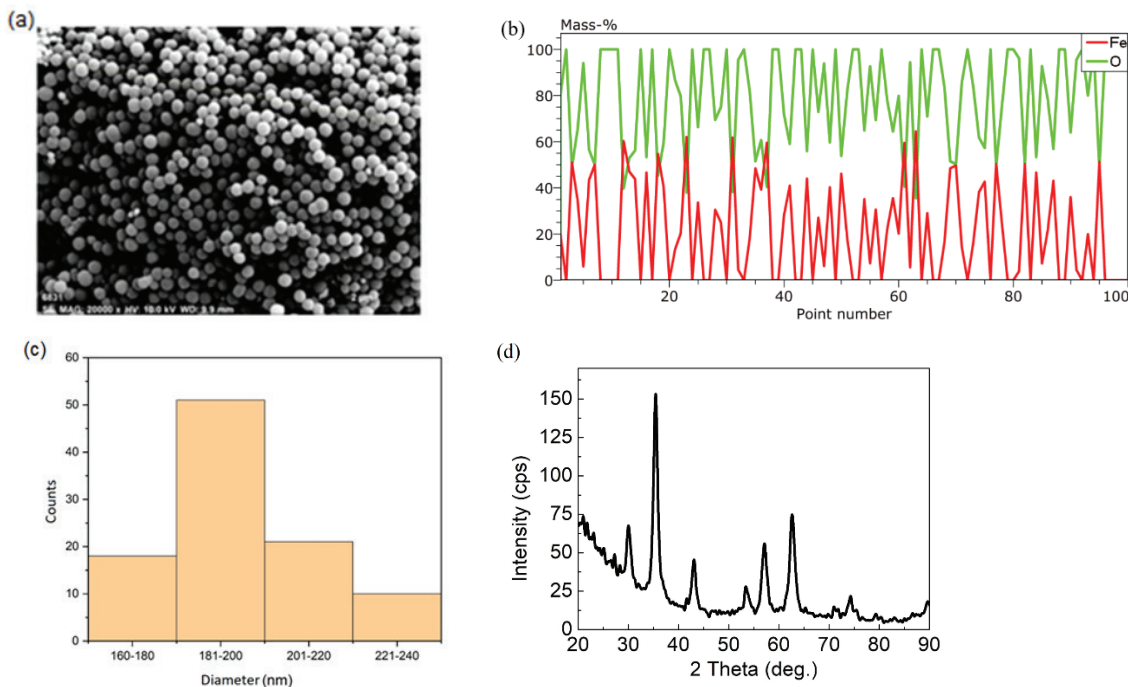
Figure 4. SEM image of the synthesized nanoparticles (a), EDX spectra (b), MNP size distribution (c), and XRD pattern of the synthesized nanoparticles (d).
