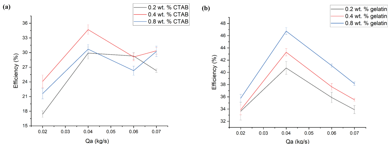
Figure 6. Thermal efficiency of WCT versus air mass flow rate for MNFs with various concentrations of (a) CTAB (b) gelatin stabilizers at a fluid volume flow rate of 0.06 \text{ m}^3/\text{h} .
