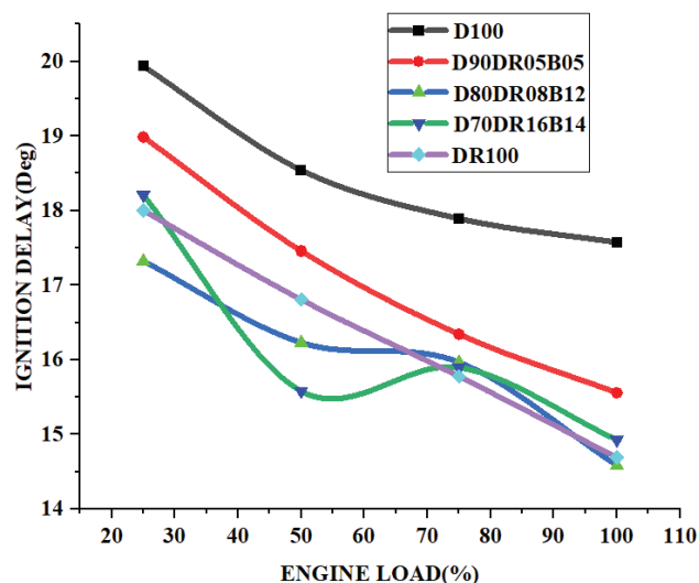
Figure 6. Ignition delay.
