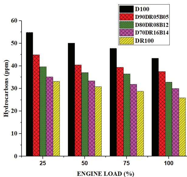
Figure 9. Hydrocarbon emissions.
