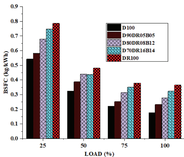
Figure 3. Specific fuel consumption vs. load.
