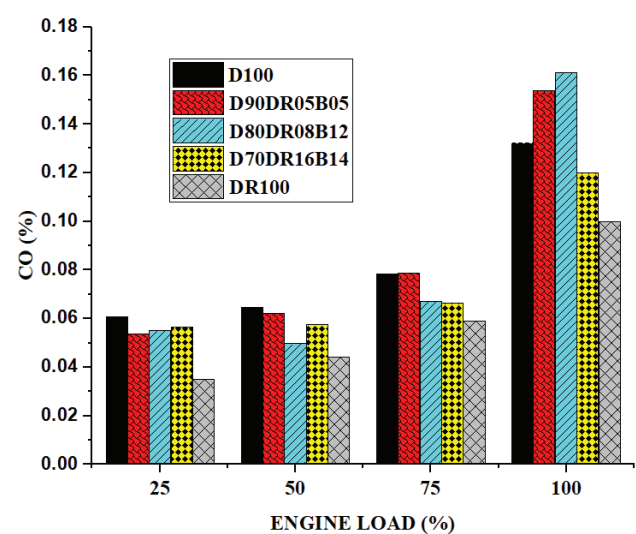
Figure 7. CO emissions.
