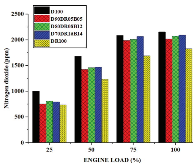
Figure 10. NO x emissions.
