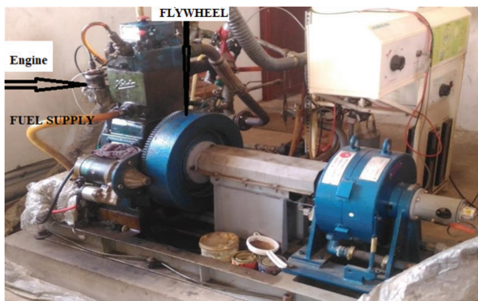
Figure 1. Actual experimental setup.
