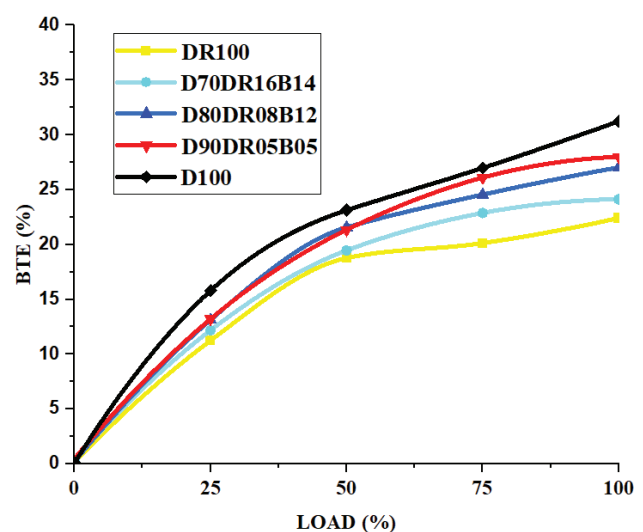
Figure 2. BTE.
