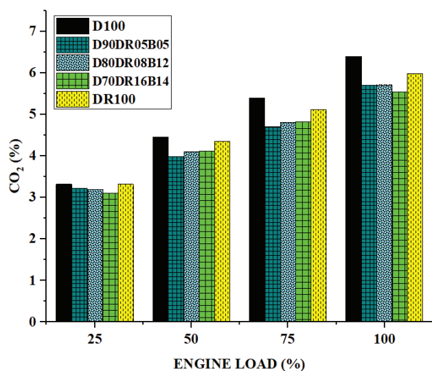
Figure 8. CO 2 emissions.
