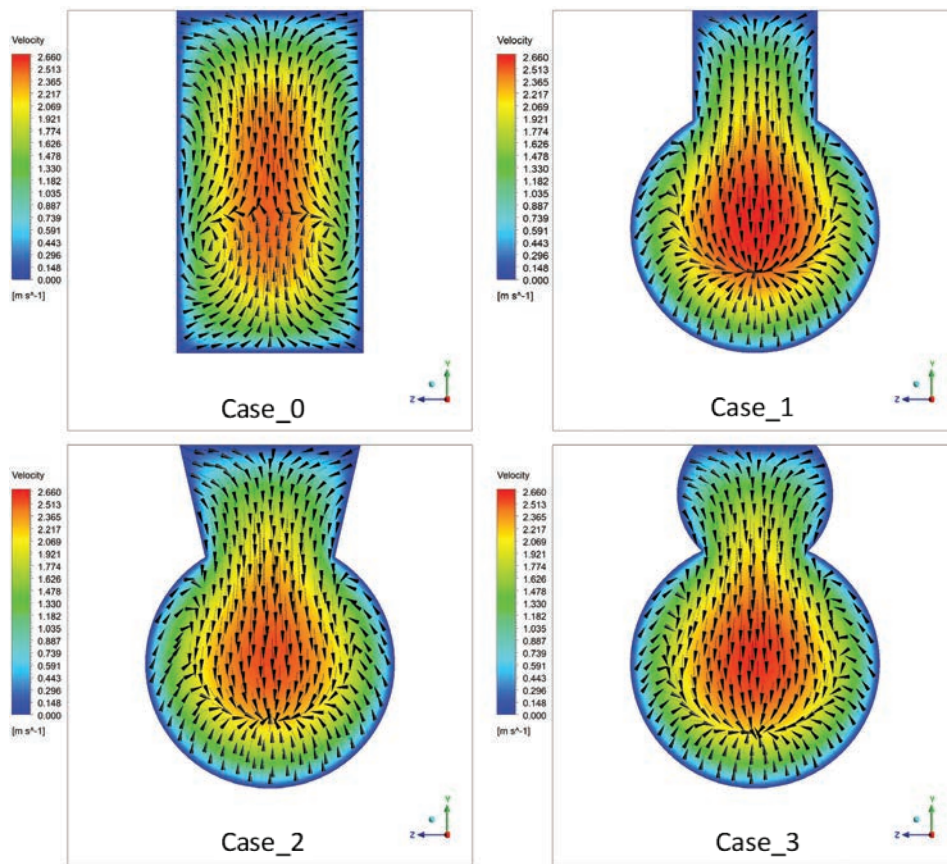
Figure 6. Streamlines and velocity contour distribution for different geometry structure on y - z plane ( x = 20 \text{ mm} ) at the outlet microchannel region with Q_{in} = 60 \text{ ml/min} for (a) \text{H}_2\text{O} , (b) \text{Al}_2\text{O}_3/\text{H}_2\text{O} , and (c) \text{CuO}/\text{H}_2\text{O} .
