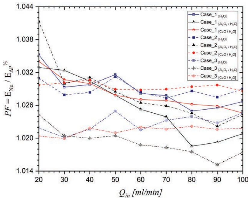
Figure 15. Variation of PF with Q_{in} for different geometry structure and different water-base nanofluids.
