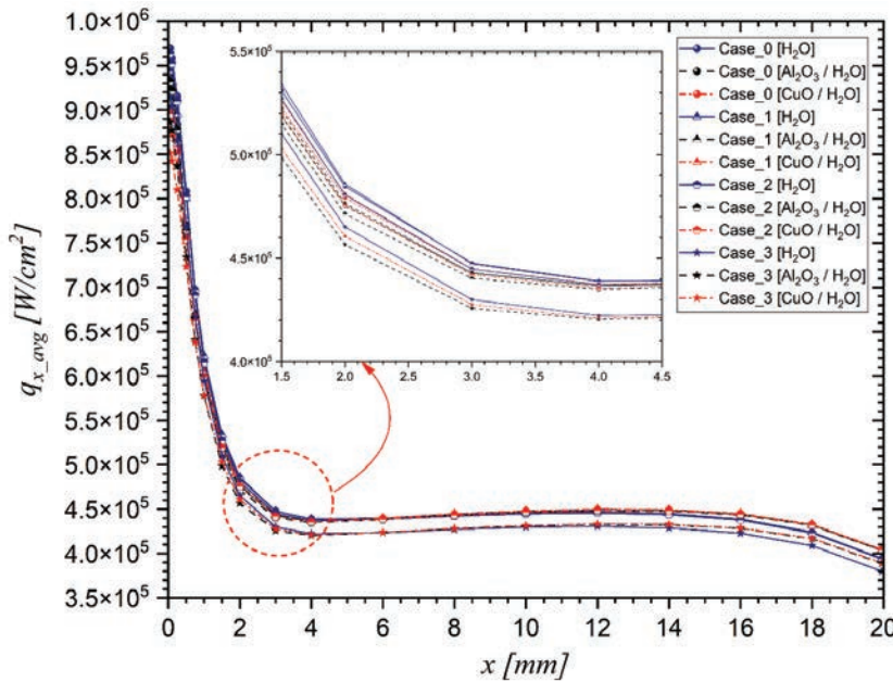
Figure 12. Comparison of the q_{x,avg} along the microchannel ( x = 0 - 20 mm) for different geometric structures and different nanofluids at Q_{in} = 60 ml/min.
