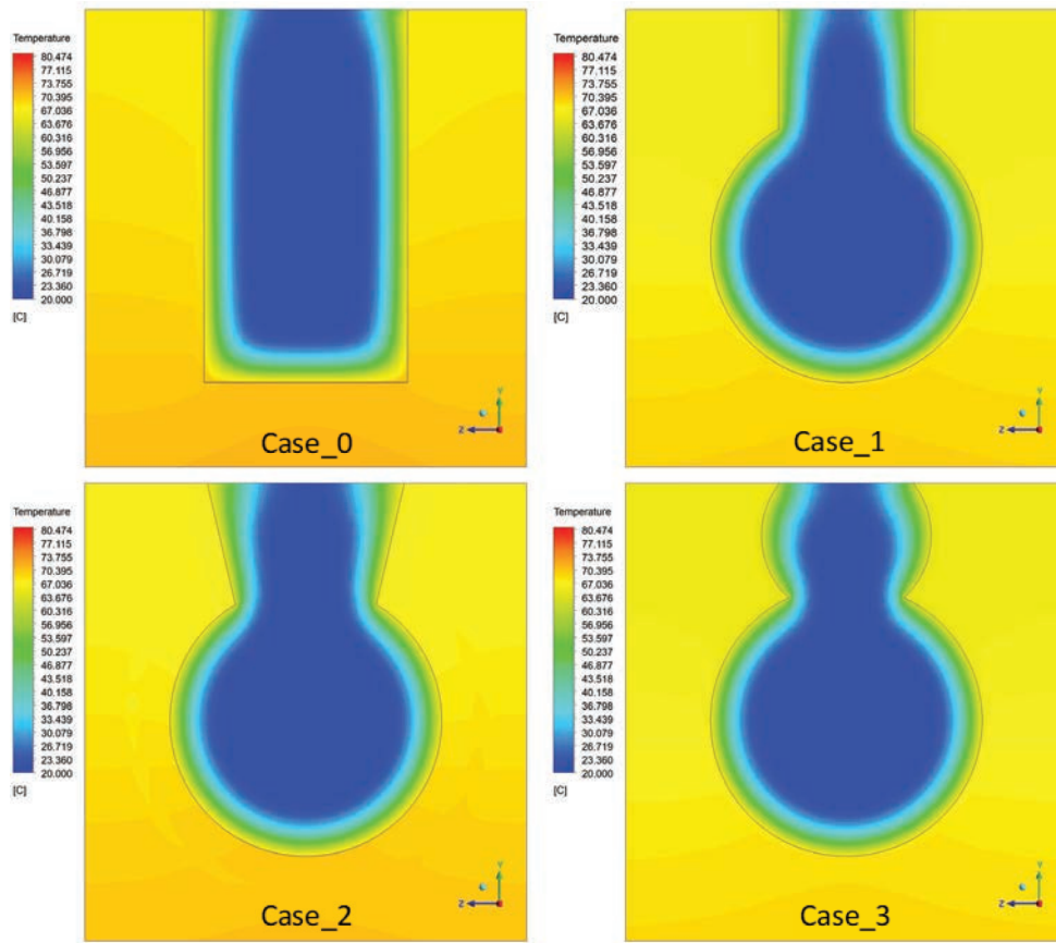
Figure 9. Comparison of 2D temperature contours for different geometric structures on the y - z plane ( x = 20 mm) at the exit region at Q_{in} = 60 ml/min for (a) H_2O , (b) Al_2O_3/H_2O , and (c) CuO/H_2O .
