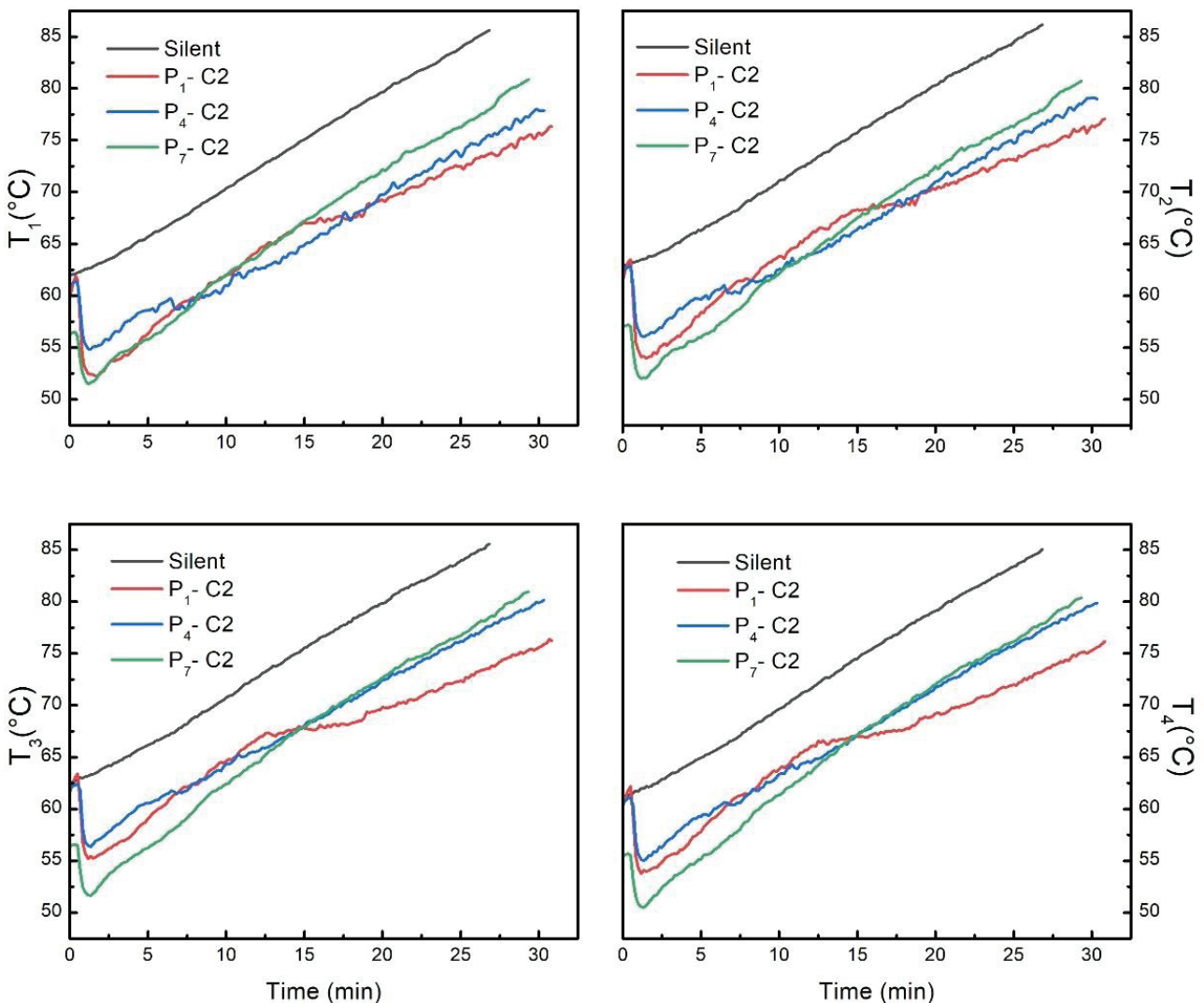
Figure 8. Evolution of the temperatures T_1 , T_2 , T_3 , and T_4 versus time for the C2 configuration cas.
