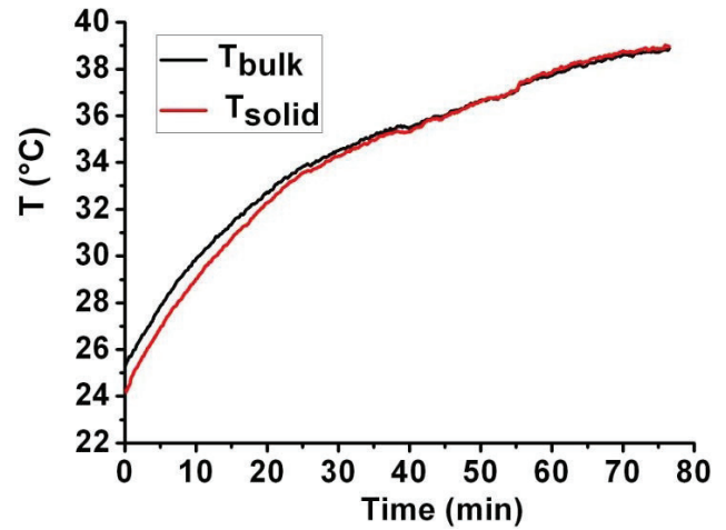
Figure 6. Evolution of water and solid temperatures versus time with two transducers in operation without heating.
