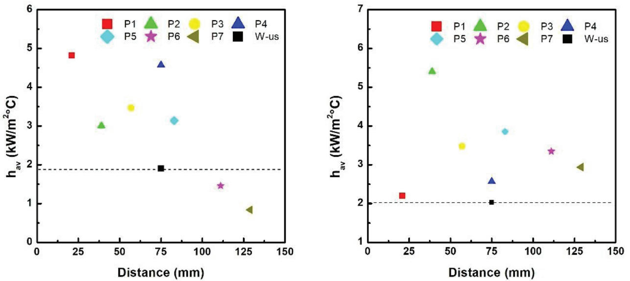
Figure 15. The average convective heat transfer coefficients versus the distance of the heat source in the tank for the C2 configuration.
