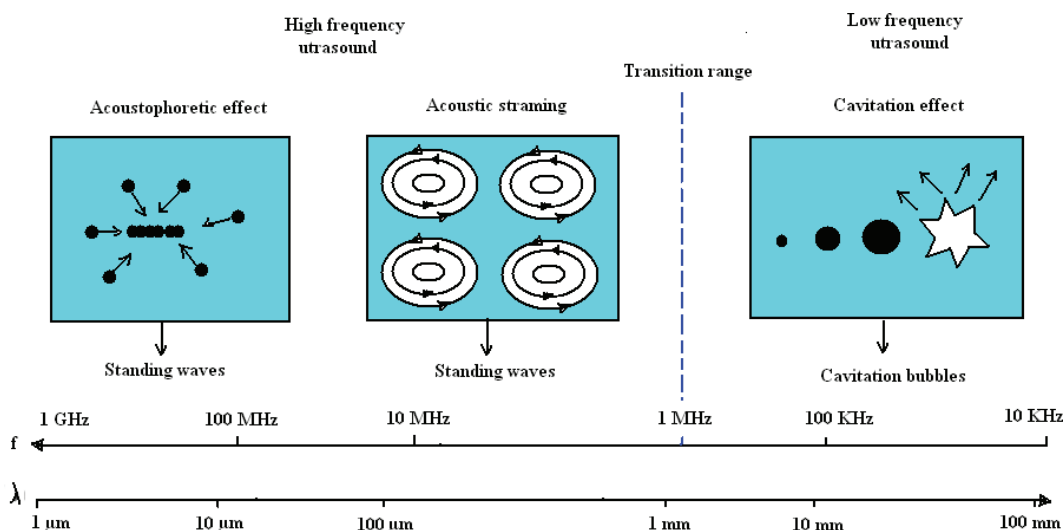
Figure 1. The different phenomena associated with high and low frequency ultrasound.
