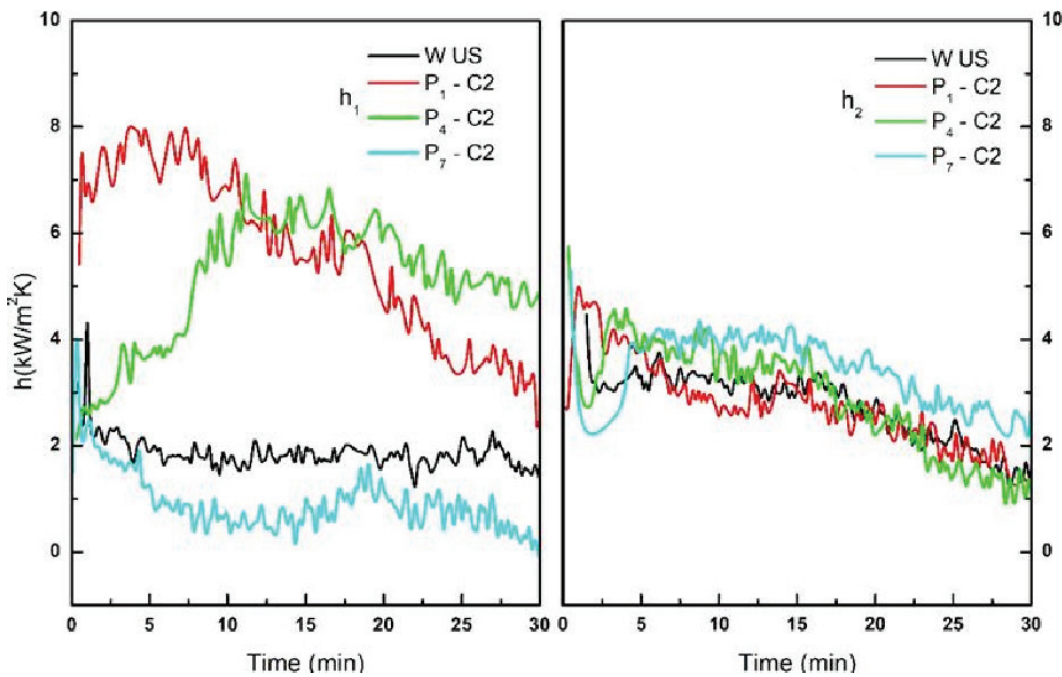
Figure 13. The local convective heat transfer coefficients versus time for the C2 configuration.
