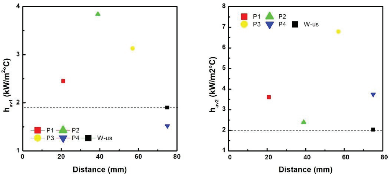
Figure 16. The average convective heat transfer coefficients versus the distance of the heat source in the tank for the C3 configuration.
