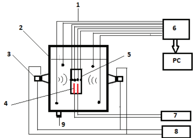
Figure 3. Schematic of the experimental device. 1- Thermocouples, 2- Tank, 3- Piezoelectric transducers, 4- Cartridge, 5- Heat source, 6- Data acquisition system, 7- DC power supply, 8- Ultrasonic generator, 9- Drainage valve.
