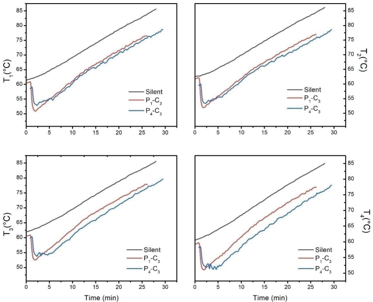
Figure 9. Temporal evolution of the wall temperatures in the C3 configuration case.
