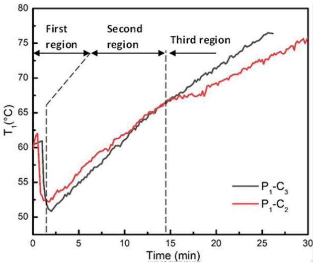
Figure 7. Evolution of the temperature T_1 versus time for C2 and C3 configurations.
