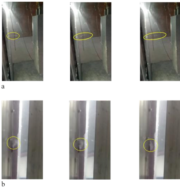
Figure 10. Propagation of the ultrasonic jet in the tank. a-position 4, b-position 1.
