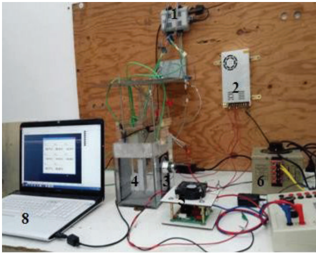
Figure 2. Picture of the experimental set-up. 1- Data acquisition, 2- DC power supply, 3- 40 KHz piezoelectric transducers, 4- Water tank, 5- Ultrasonic generator, 6- Voltage variator, 7- Wattmeter, 8- PC.
