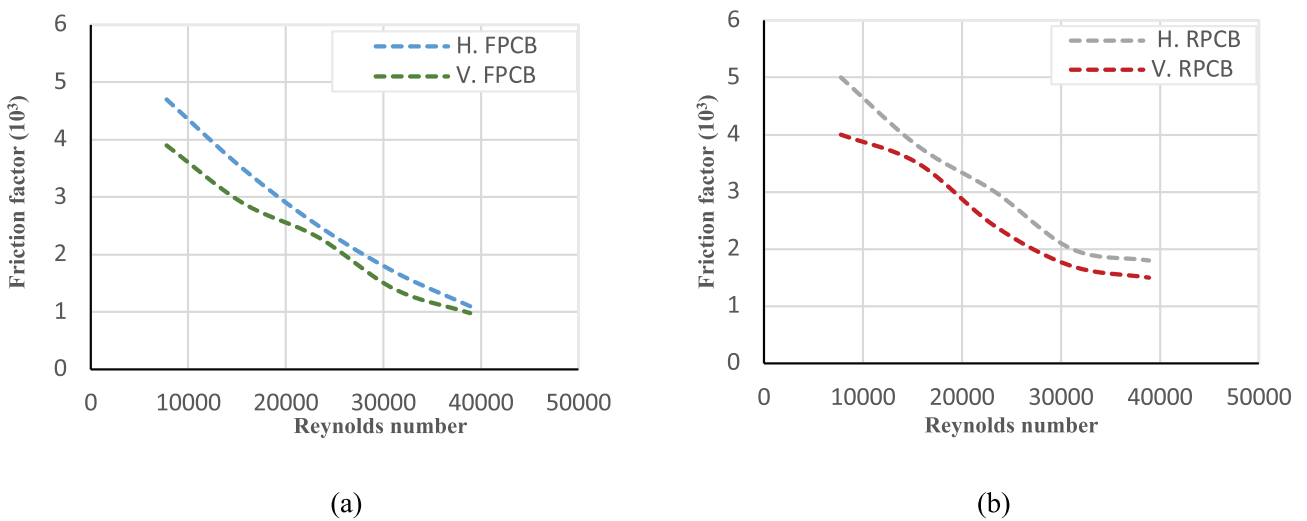
Figure 21. a) FPCB variation of numerical friction factor with Reynolds numbers at different orientations b) RPCB variation of numerical friction factor with Reynolds numbers at different orientations.
