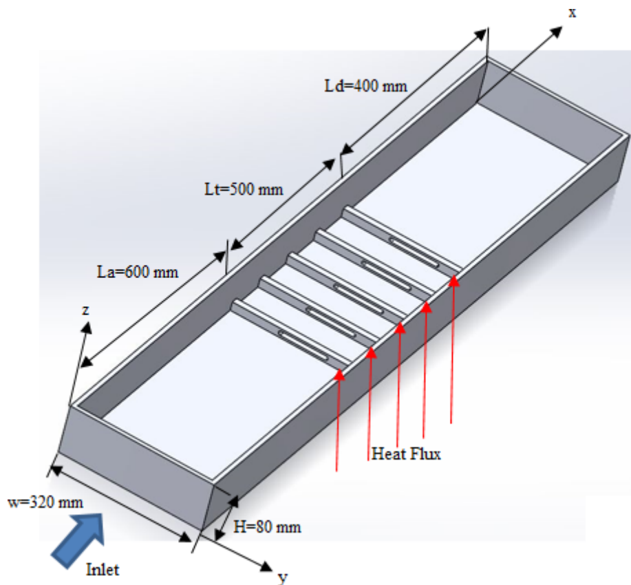
Figure 6. The rectangular channel with an array of slit ribs on the bottom of the heated section. The slit ribs have different rib height ( e= 10 \text{ mm} , 15 \text{ mm} and 20 \text{ mm} ) and slit length ( L_s/L_r = 0, 0.20, 0.35, 0.50 ) (modified from [13]).
