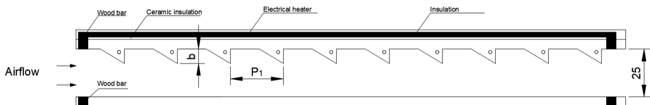
Figure 14. Test section mounted with PWs (modified from [32]).
